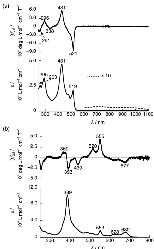
Figure 2. MCD (top) and UV/Vis absorption (bottom) spectra of a) \text{Ni}^{\text{II}} norcorrole 2 and b) \text{Ni}^{\text{II}} oxacorrole 3 in \text{CH}_2\text{Cl}_2 .
